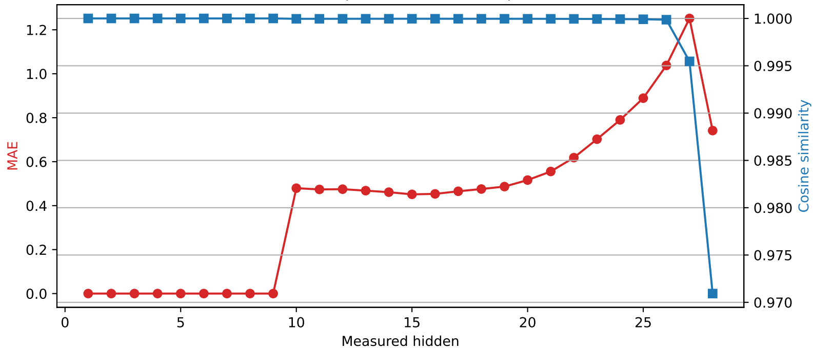
Qwen2.5-7B-Instruct | Quantized layer 9 | float32 → int2
