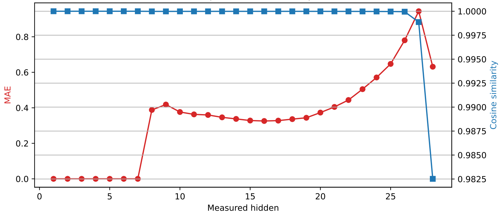
Qwen2.5-7B-Instruct | Quantized layer 7 | float64 → int2
