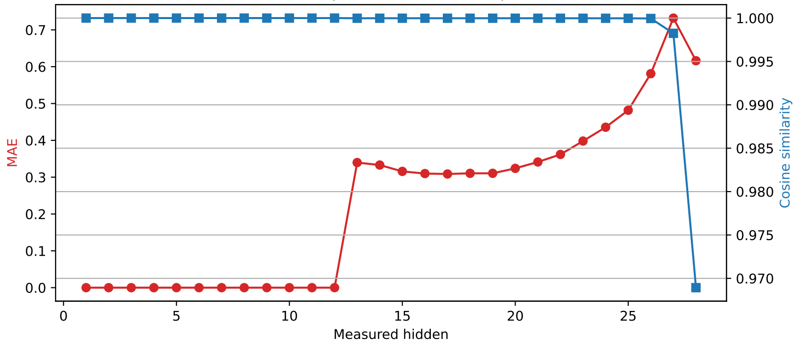
Qwen2.5-7B-Instruct | Quantized layer 12 | float64 → int2
