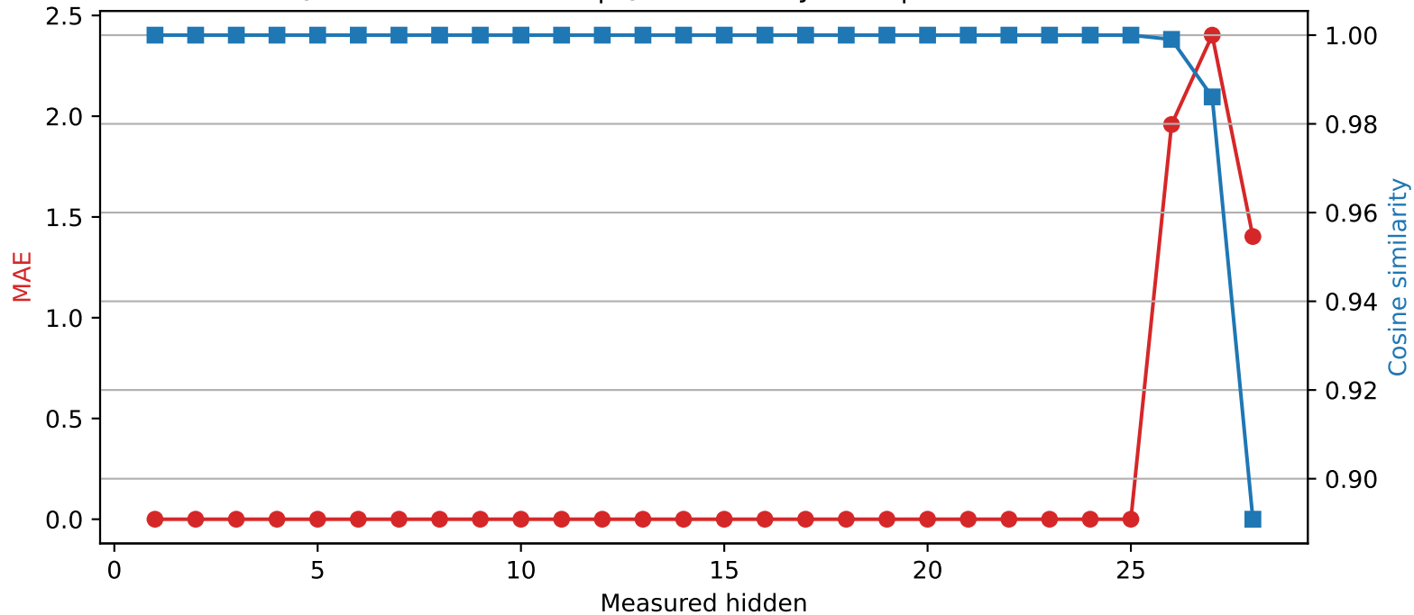
Qwen2.5-7B-Instruct | Quantized layer 25 | float64 → int2
