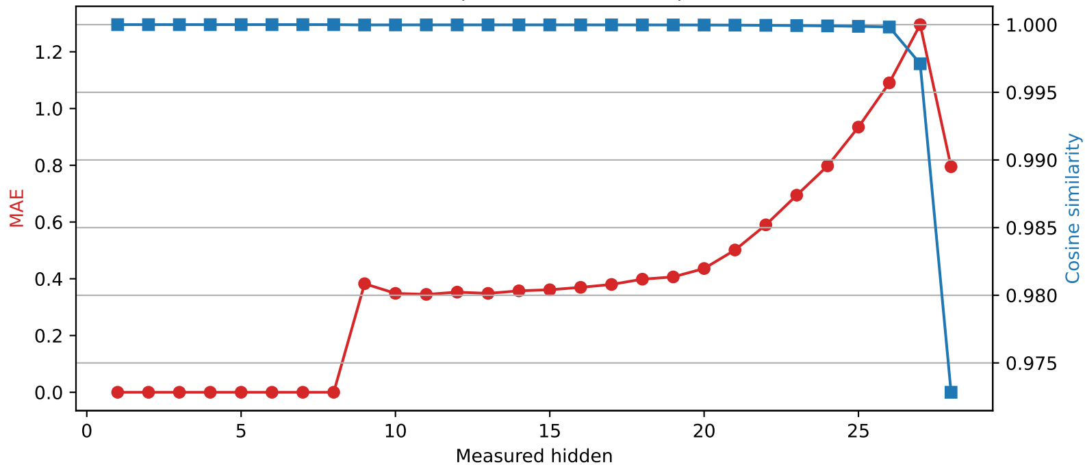
Qwen2.5-7B-Instruct | Quantized layer 8 | float64 → int2
