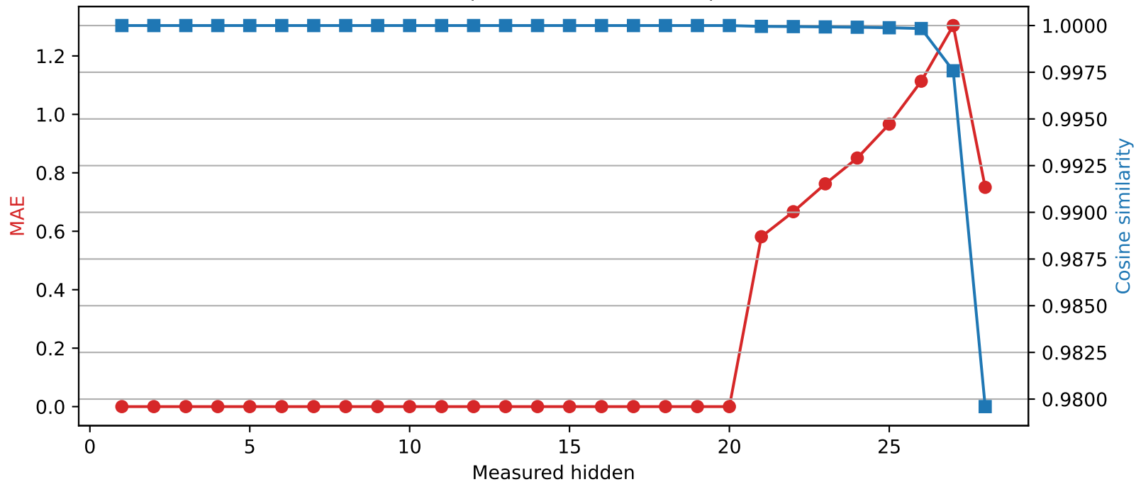
Qwen2.5-7B-Instruct | Quantized layer 20 | float64 → int2
