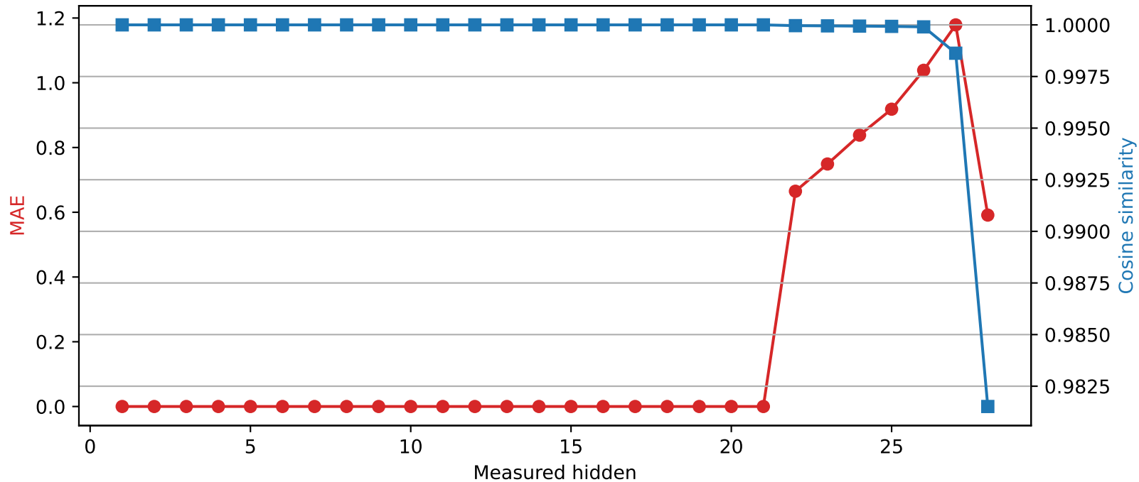
Qwen2.5-7B-Instruct | Quantized layer 21 | float64 → int2
