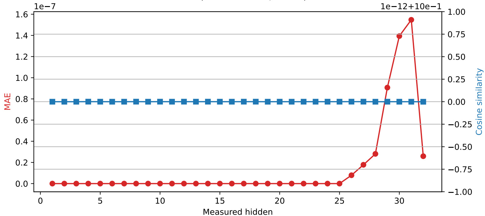
Phi-3-mini-4k-instruct | Quantized layer 25 | float64 → int32
