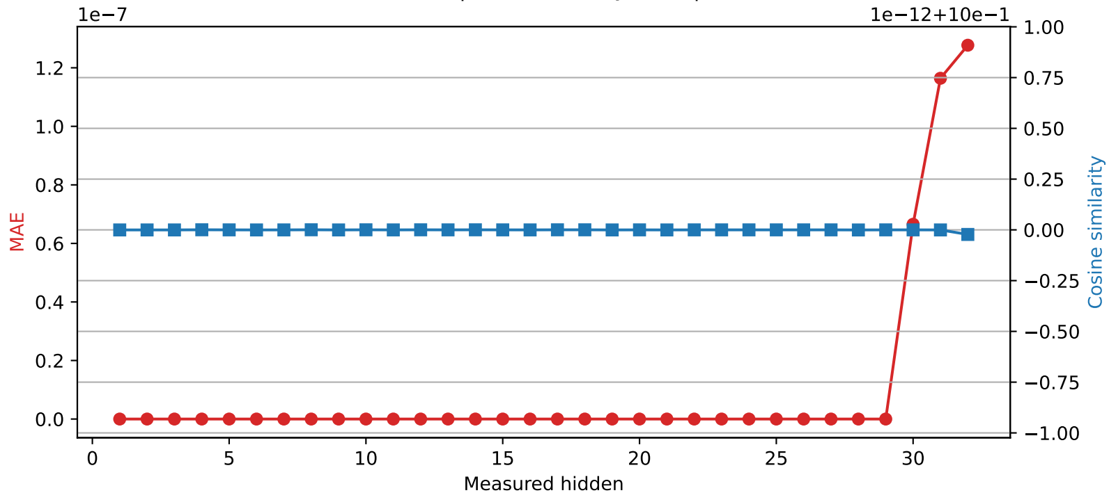
Phi-3-mini-4k-instruct | Quantized layer 29 | float64 → int32
