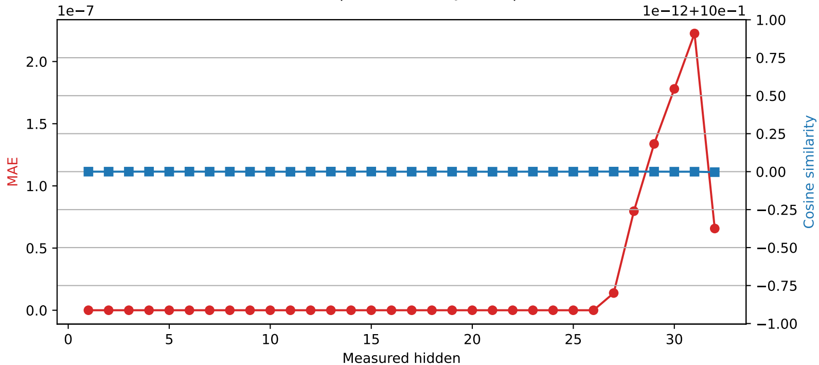
Phi-3-mini-4k-instruct | Quantized layer 26 | float64 → int32
