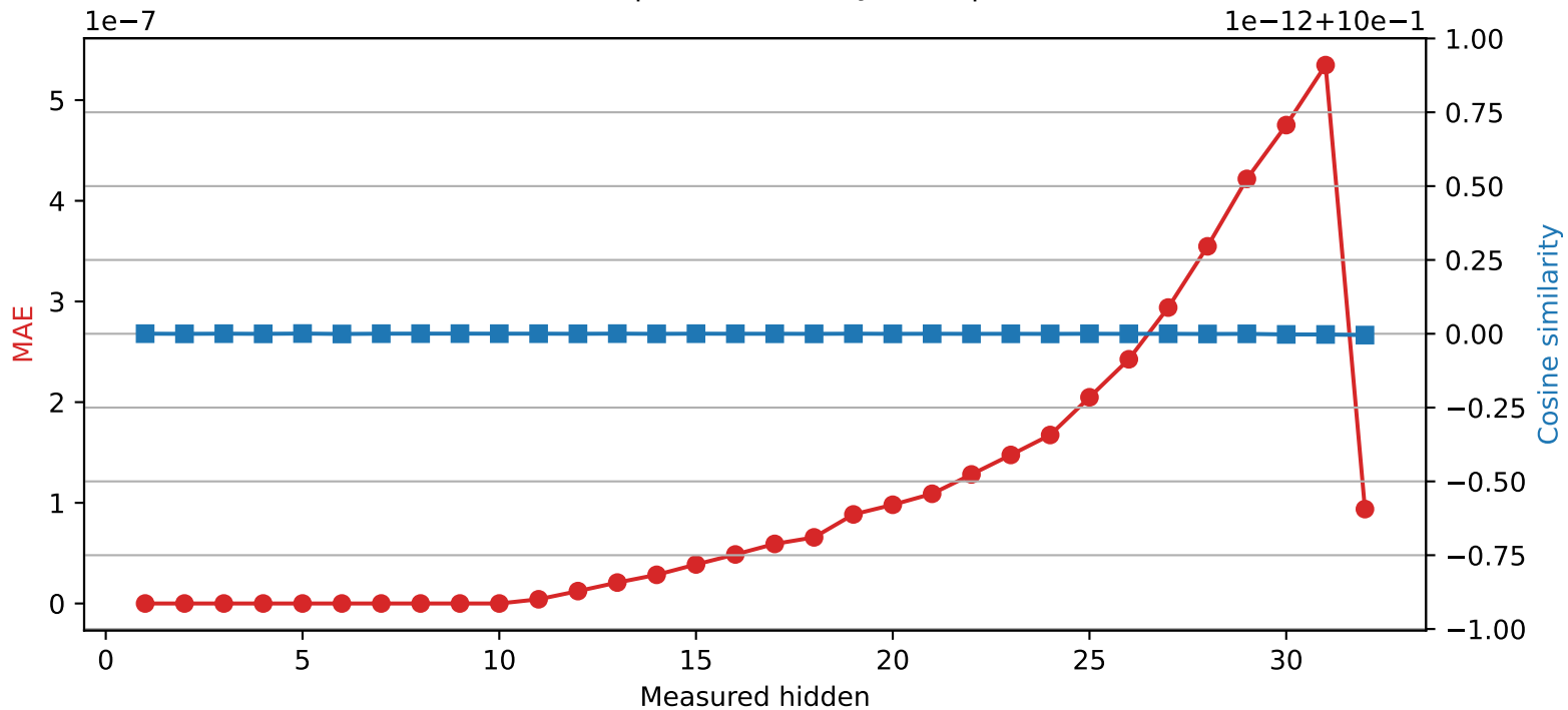
Phi-3-mini-4k-instruct | Quantized layer 10 | float64 → int32
