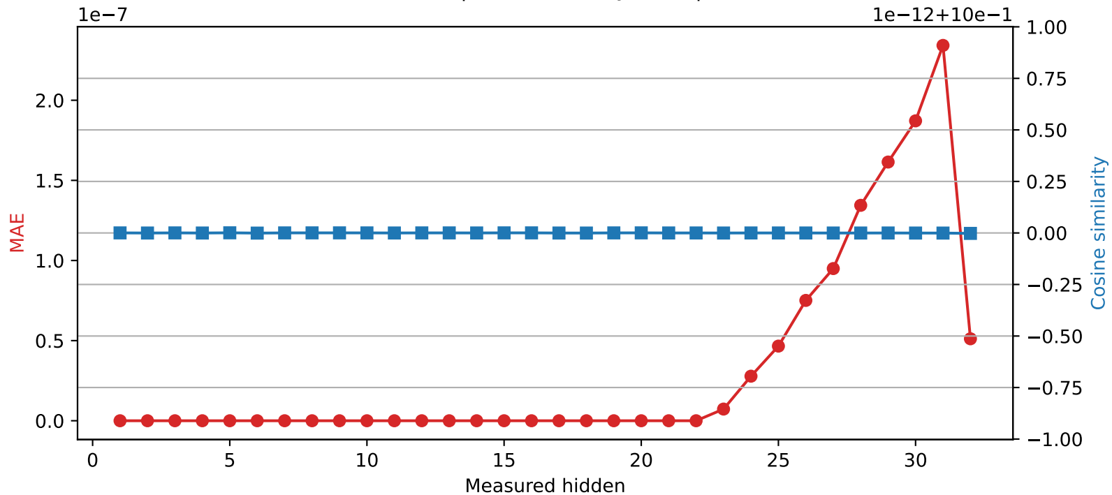
Phi-3-mini-4k-instruct | Quantized layer 22 | float64 → int32
