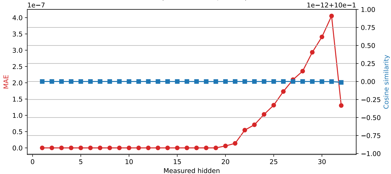
Phi-3-mini-4k-instruct | Quantized layer 19 | float64 → int32
