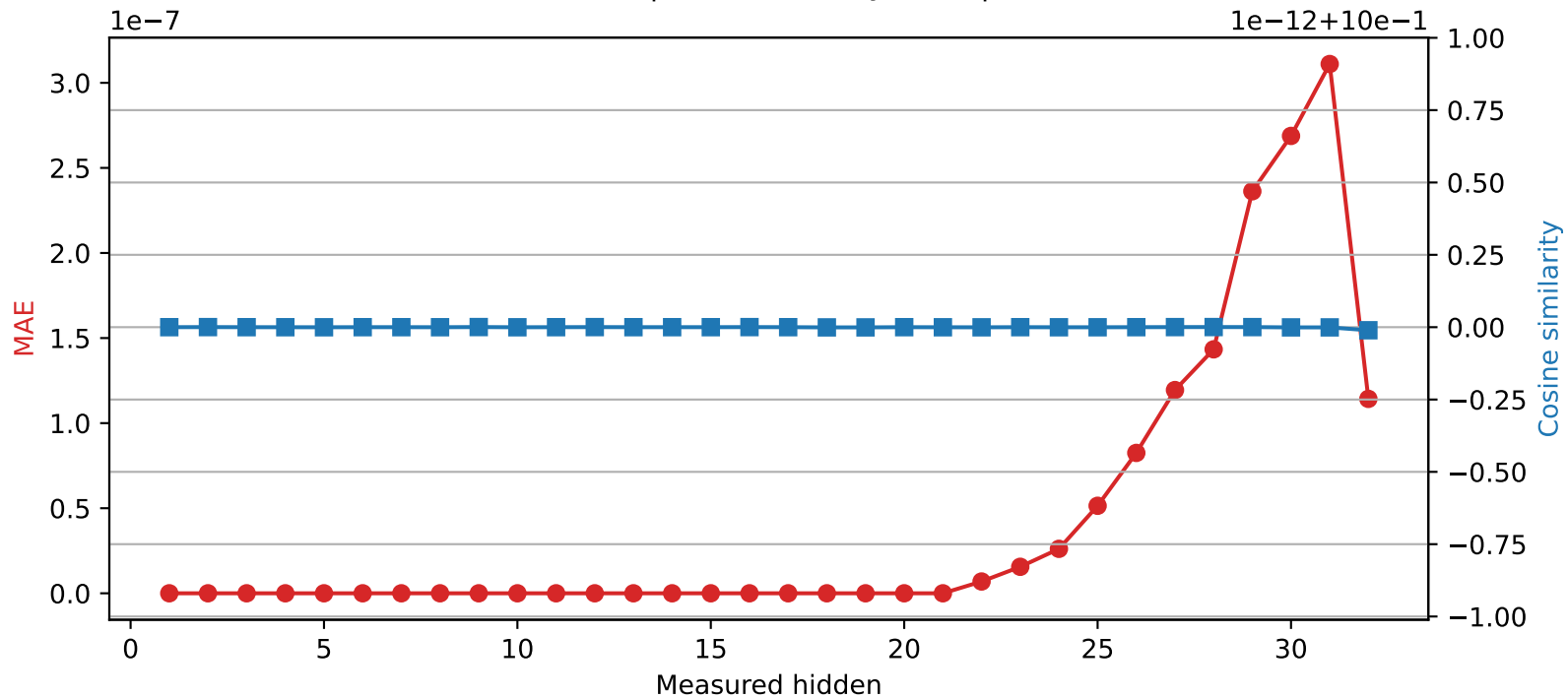
Phi-3-mini-4k-instruct | Quantized layer 21 | float64 → int32
