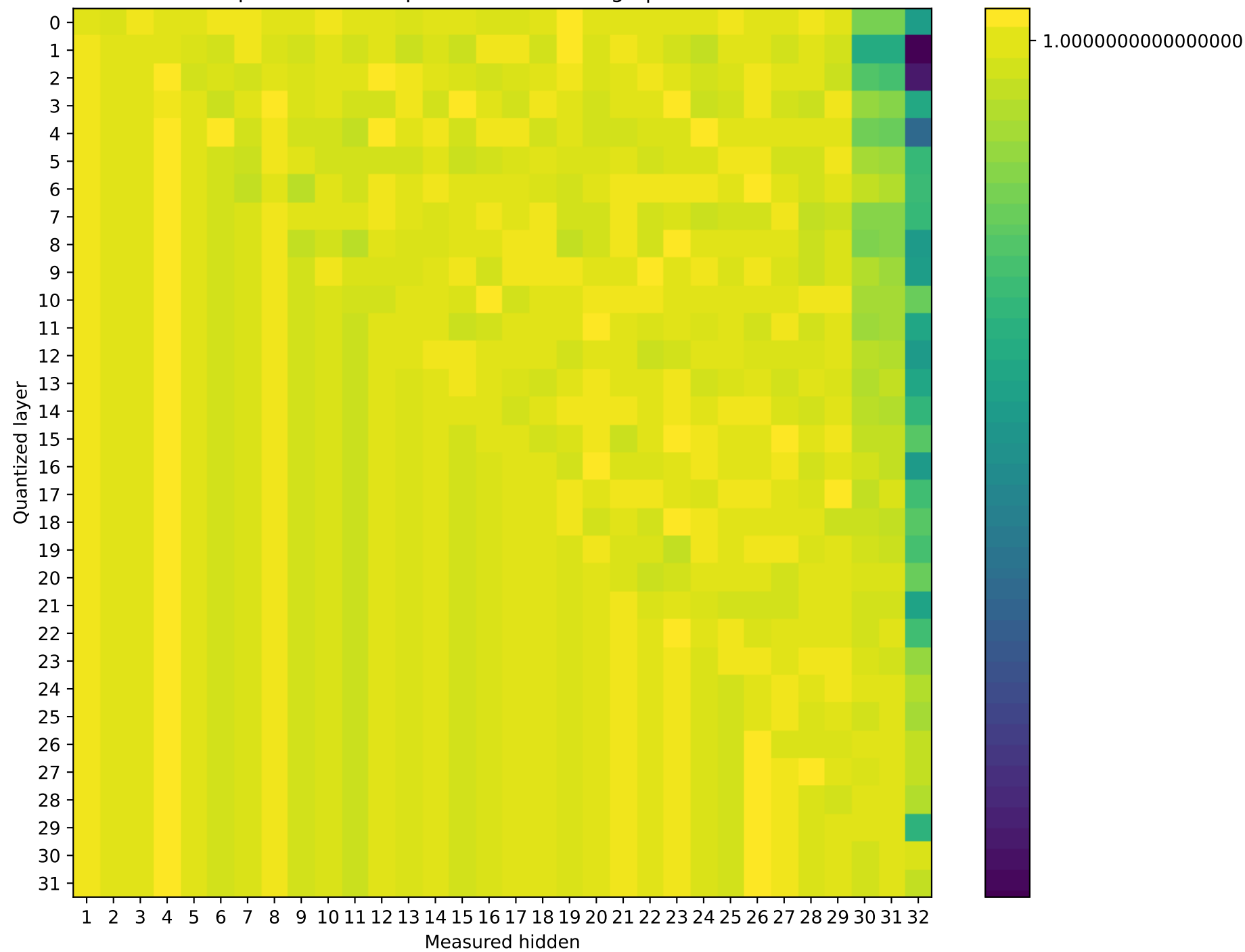
Phi-3-mini-4k-instruct Prompt 4: cos sim representation damage | float64 → int32
