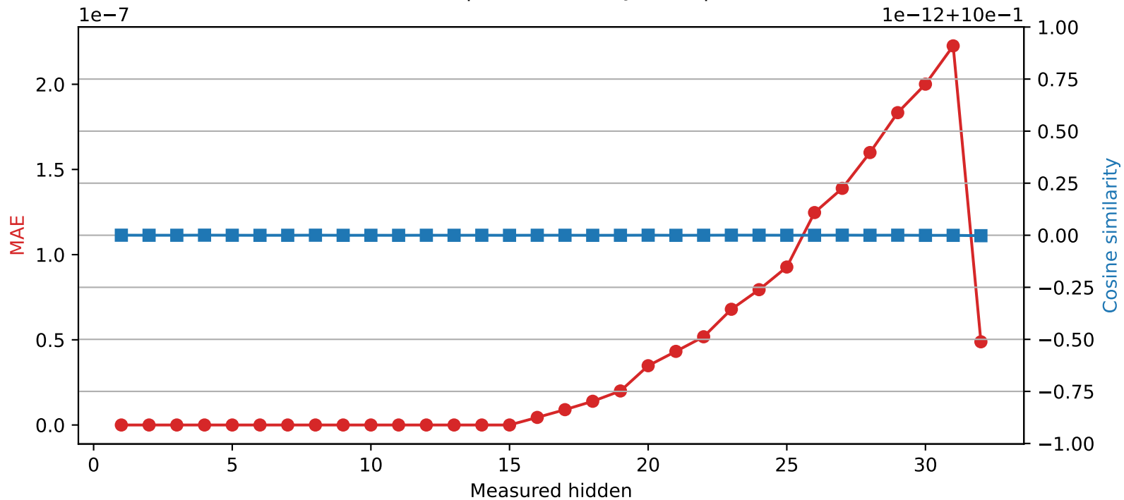
Phi-3-mini-4k-instruct | Quantized layer 15 | float64 → int32
