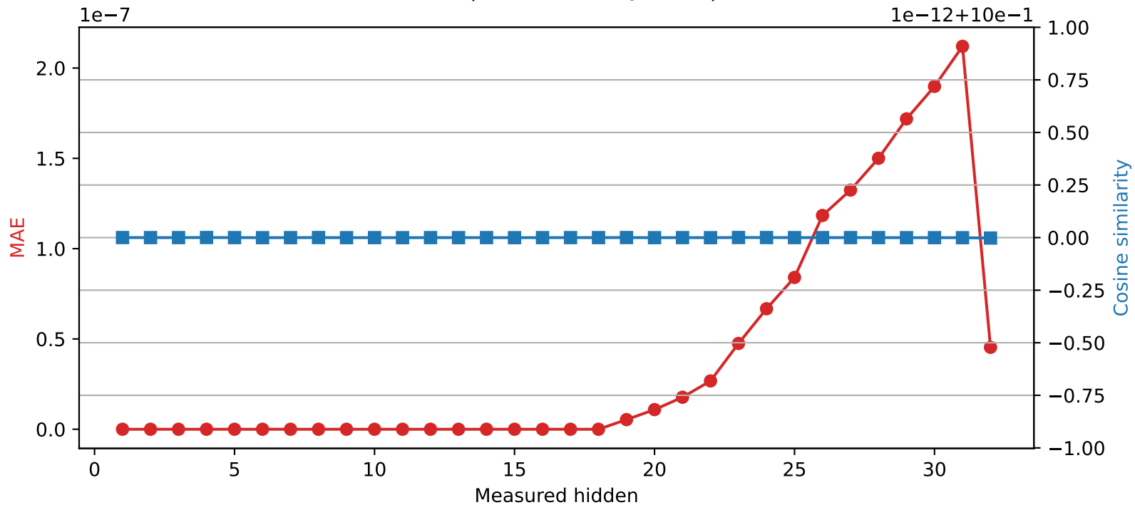
Phi-3-mini-4k-instruct | Quantized layer 18 | float64 → int32
