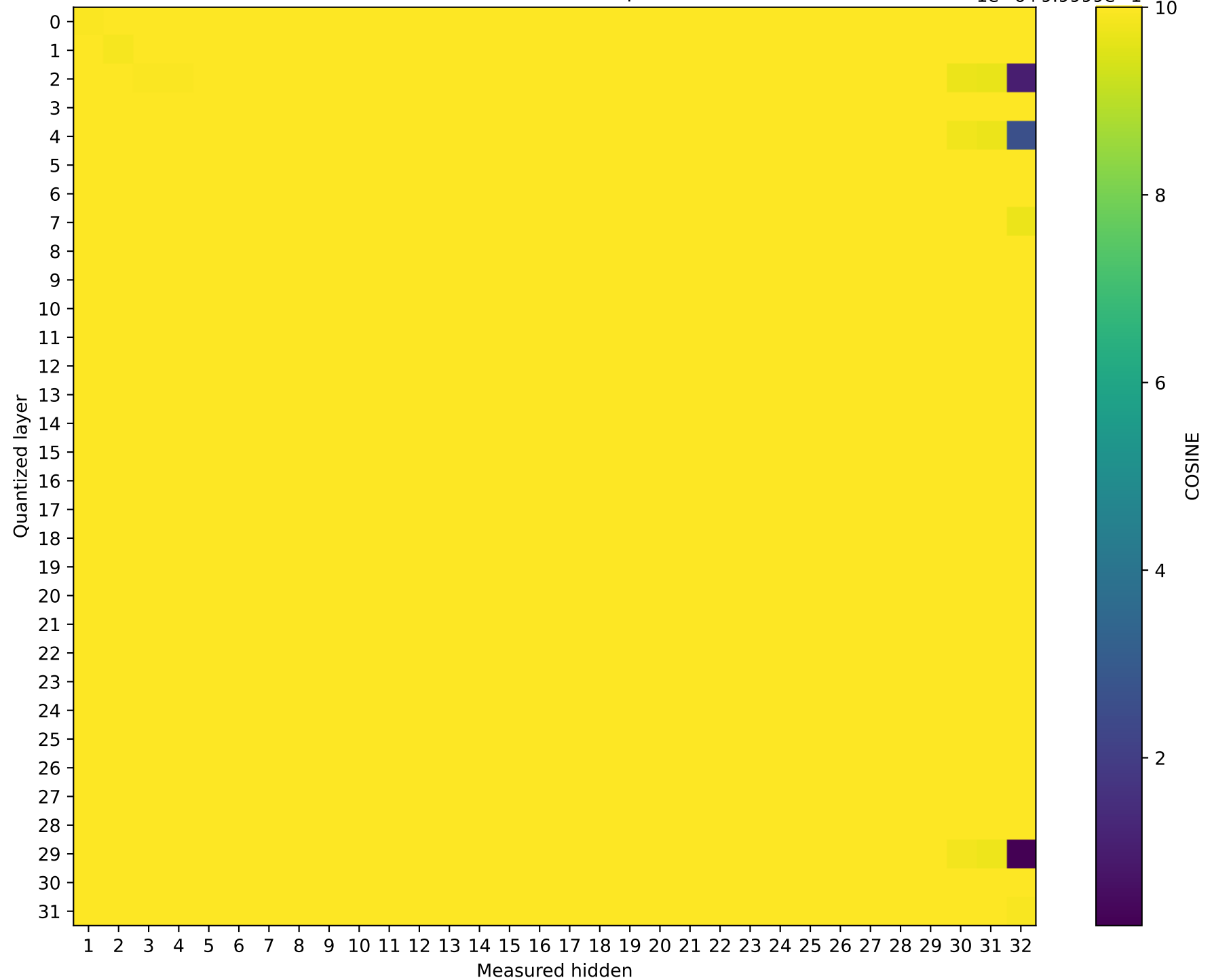
Model: Phi-3-mini-4k-instruct | float32 → int16
