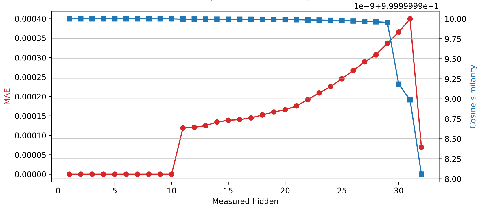
Phi-3-mini-4k-instruct | Quantized layer 10 | float32 → int16
