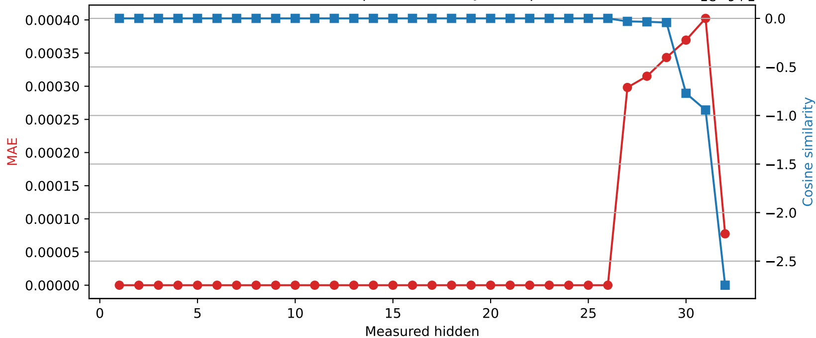
Phi-3-mini-4k-instruct | Quantized layer 26 | float32 \rightarrow int16
