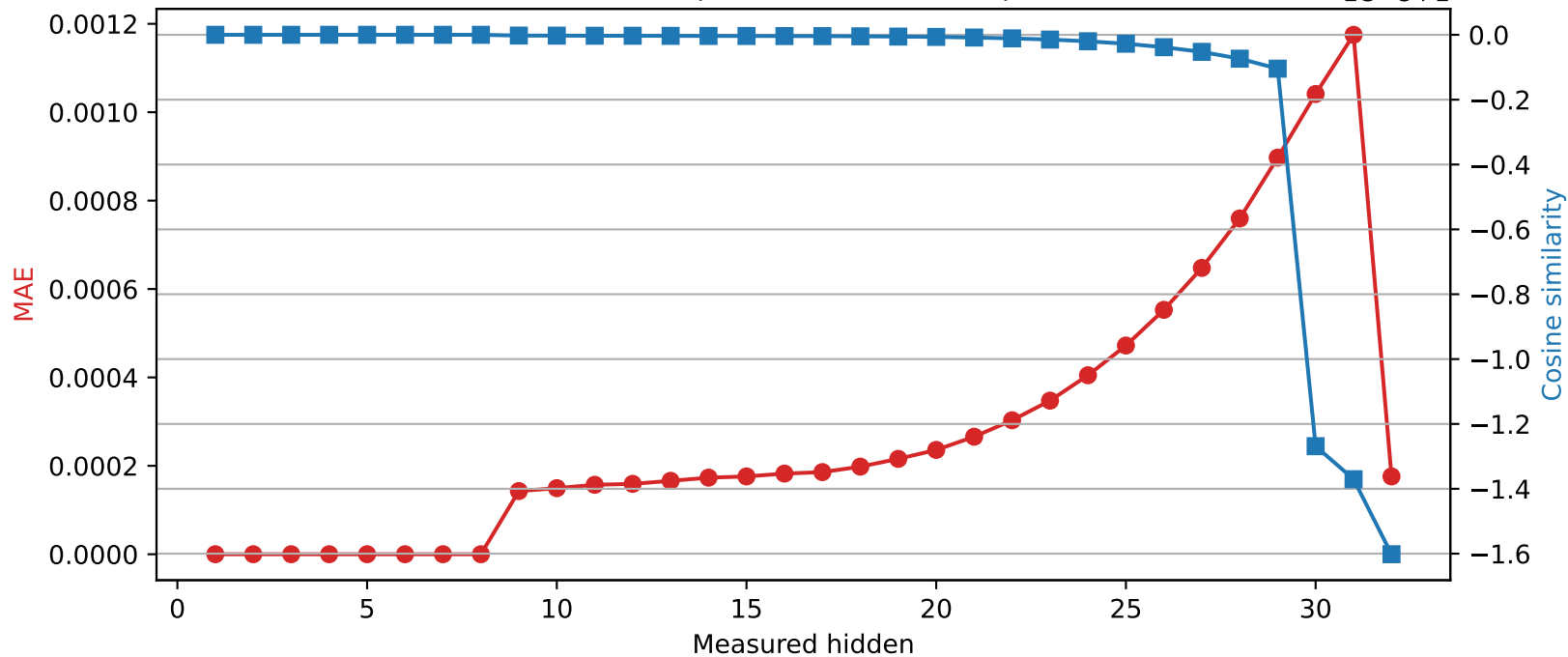
Phi-3-mini-4k-instruct | Quantized layer 8 | float32 \rightarrow int16
