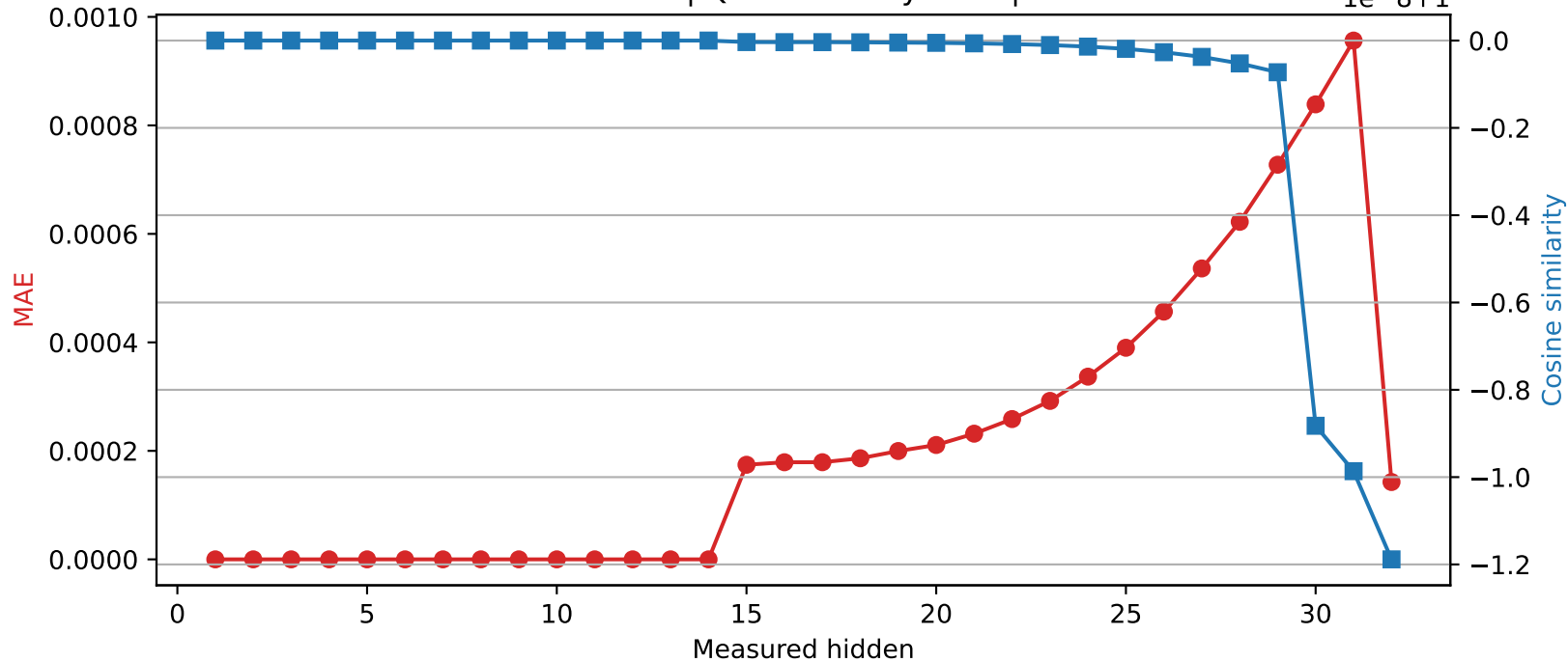
Phi-3-mini-4k-instruct | Quantized layer 14 | float32 \rightarrow int16
