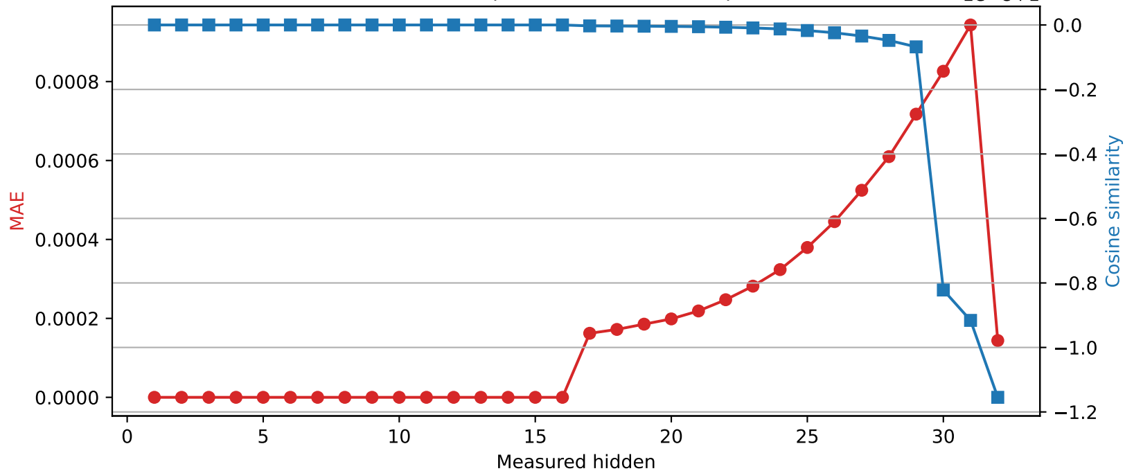
Phi-3-mini-4k-instruct | Quantized layer 16 | float32 \rightarrow int16
