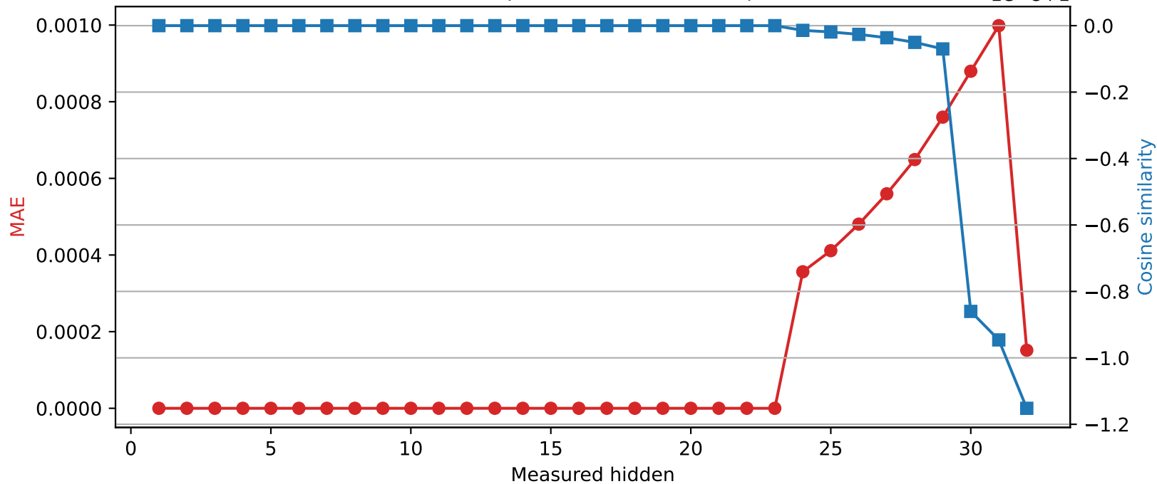
Phi-3-mini-4k-instruct | Quantized layer 23 | float32 \rightarrow int16
