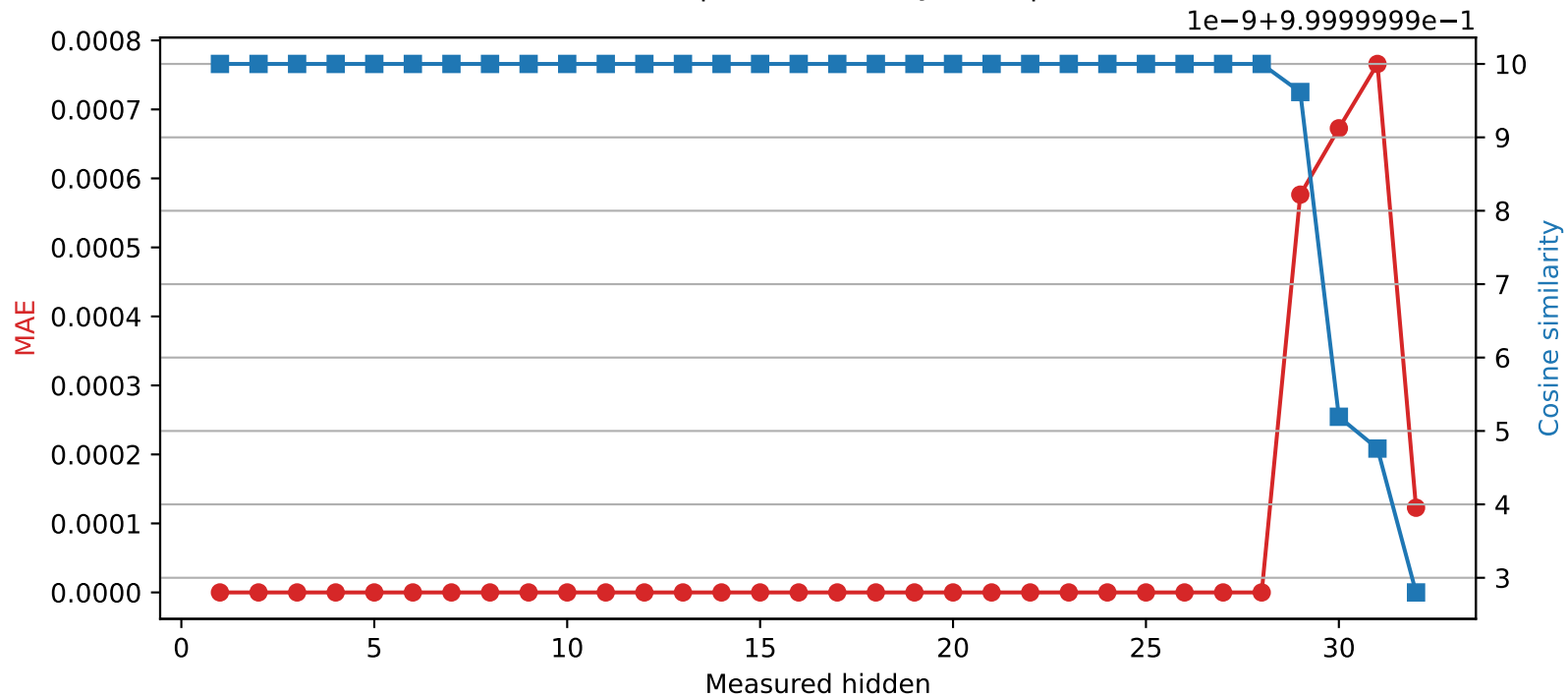
Phi-3-mini-4k-instruct | Quantized layer 28 | float32 → int16
