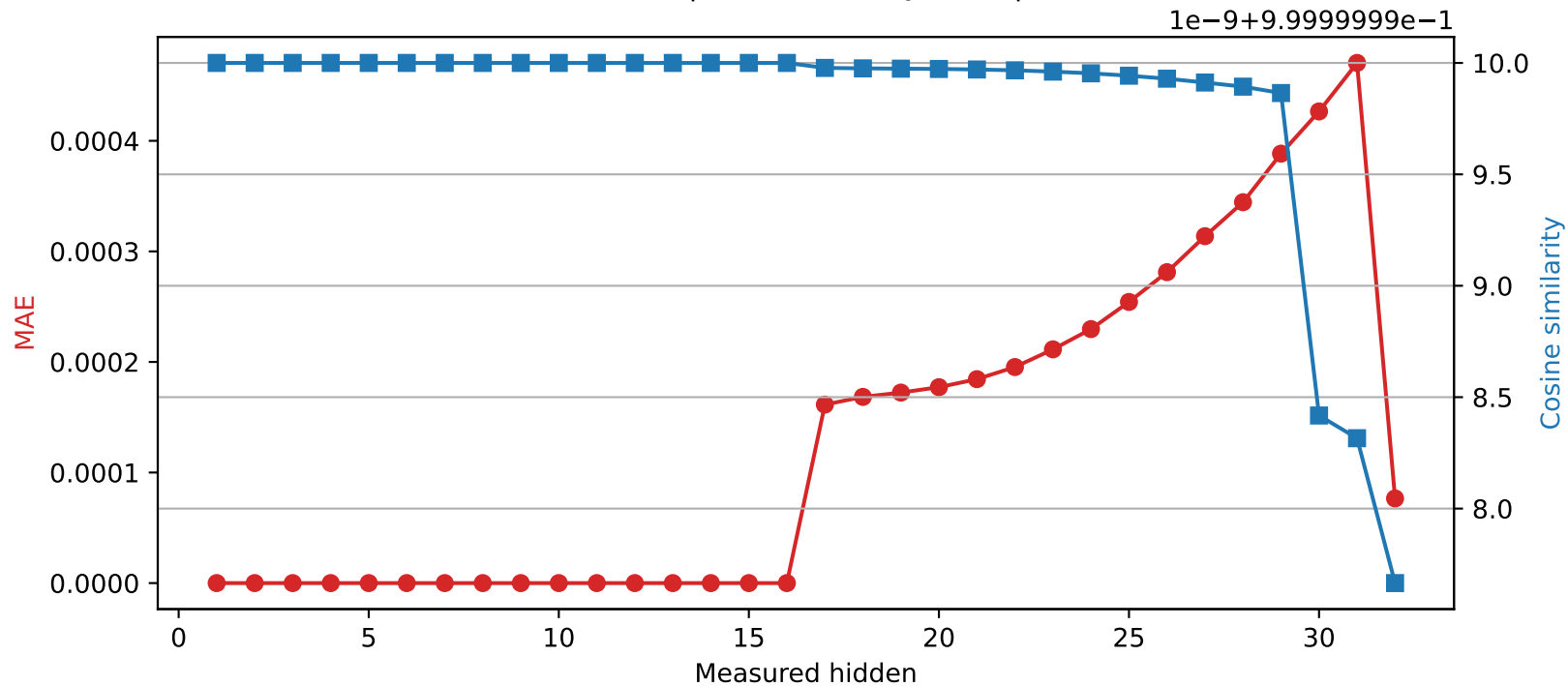
Phi-3-mini-4k-instruct | Quantized layer 16 | float32 → int16
