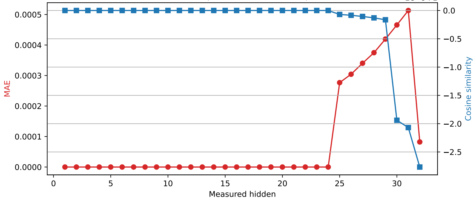
Phi-3-mini-4k-instruct | Quantized layer 24 | float32 \rightarrow int16
