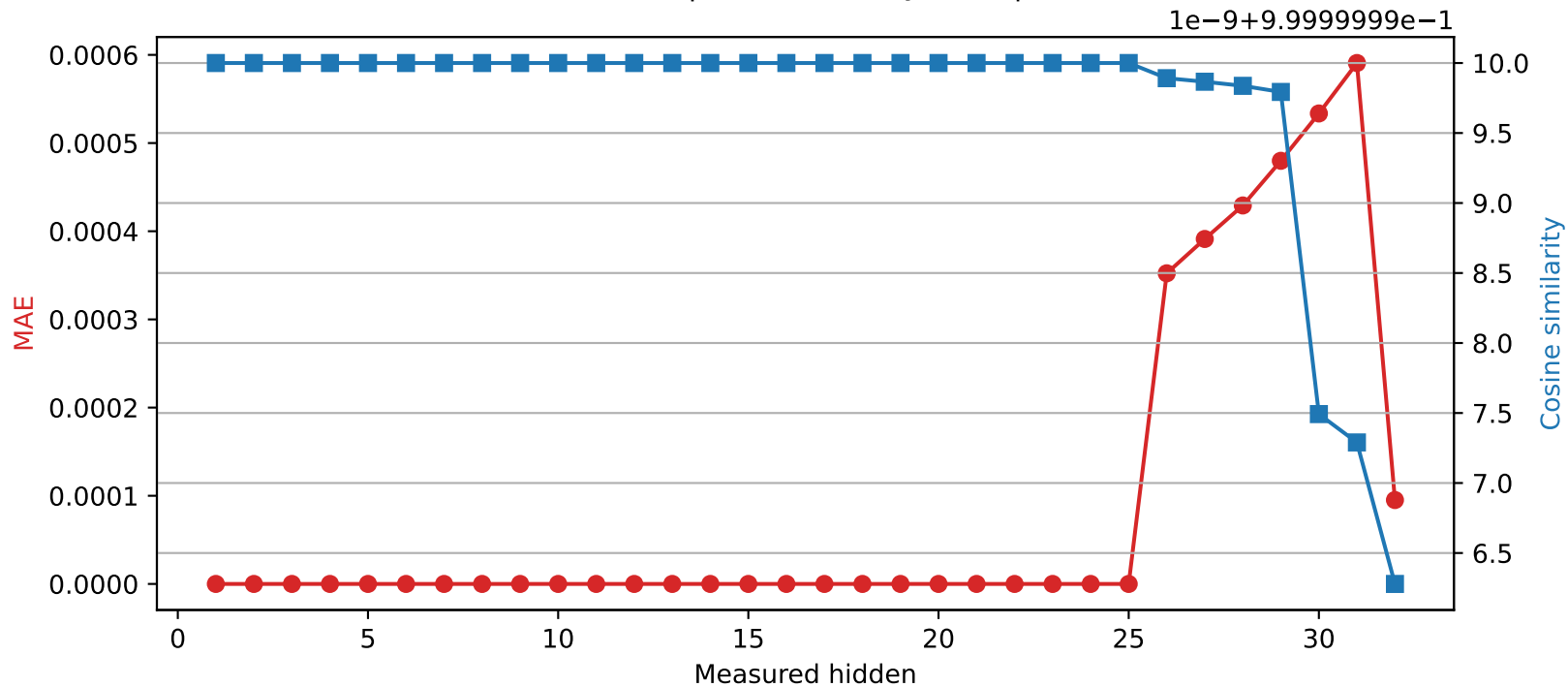
Phi-3-mini-4k-instruct | Quantized layer 25 | float32 → int16
