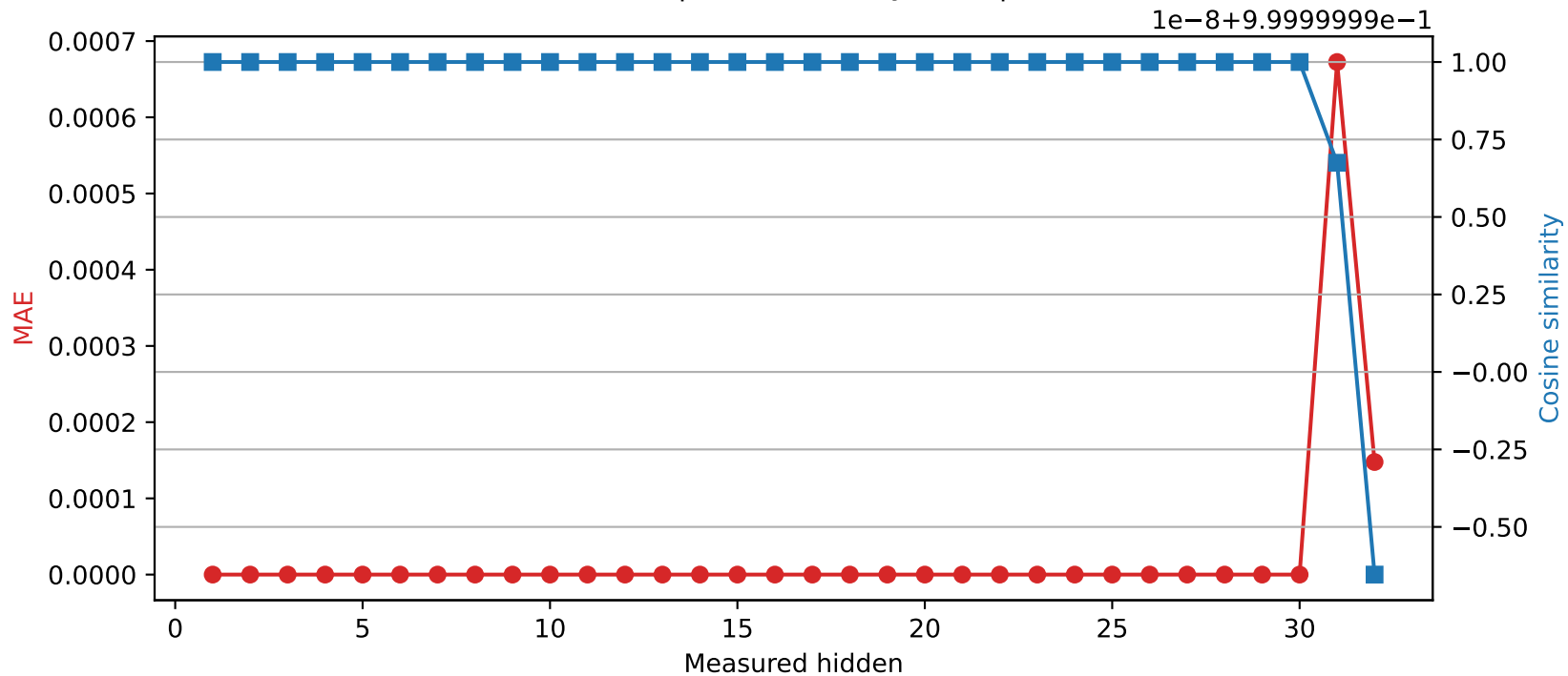
Phi-3-mini-4k-instruct | Quantized layer 30 | float32 → int16
