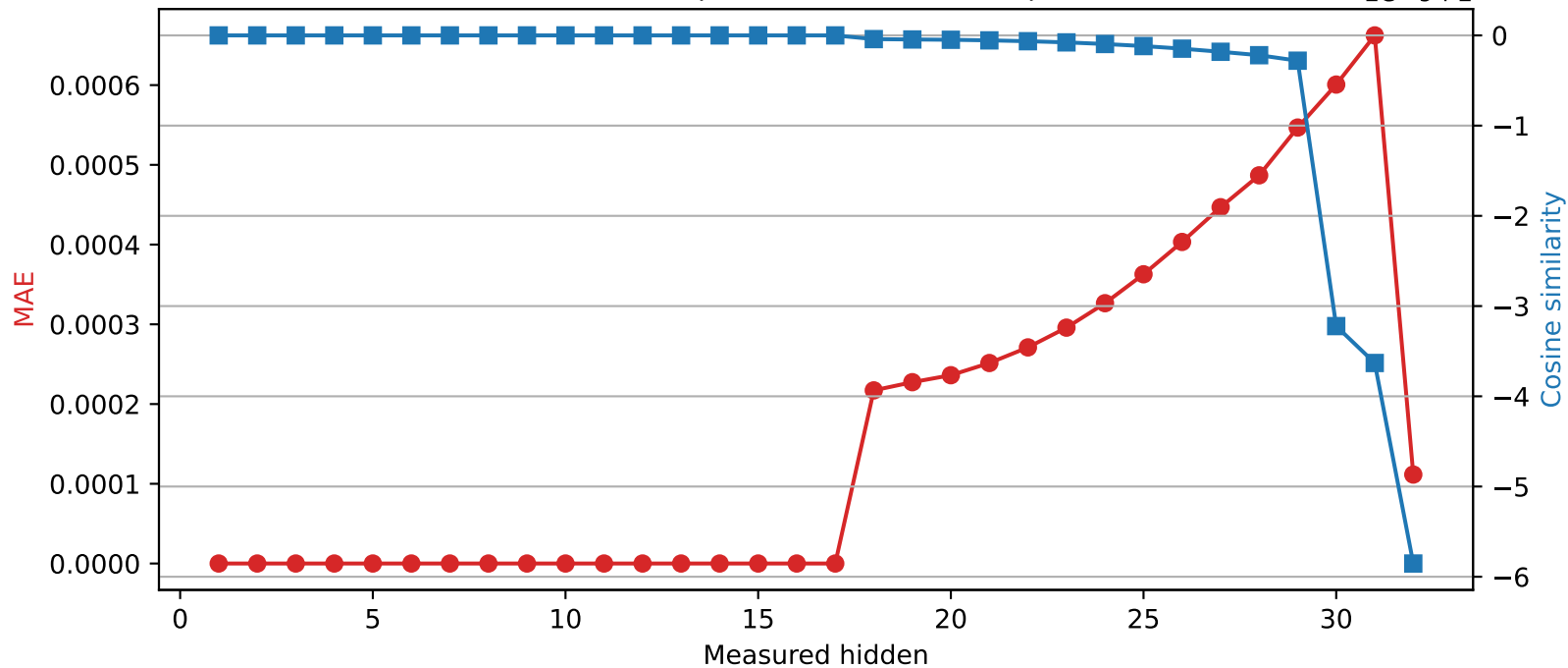
Phi-3-mini-4k-instruct | Quantized layer 17 | float32 \rightarrow int16
