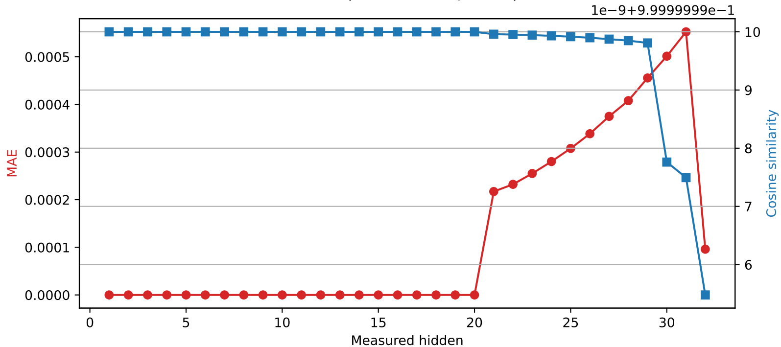
Phi-3-mini-4k-instruct | Quantized layer 20 | float32 → int16
