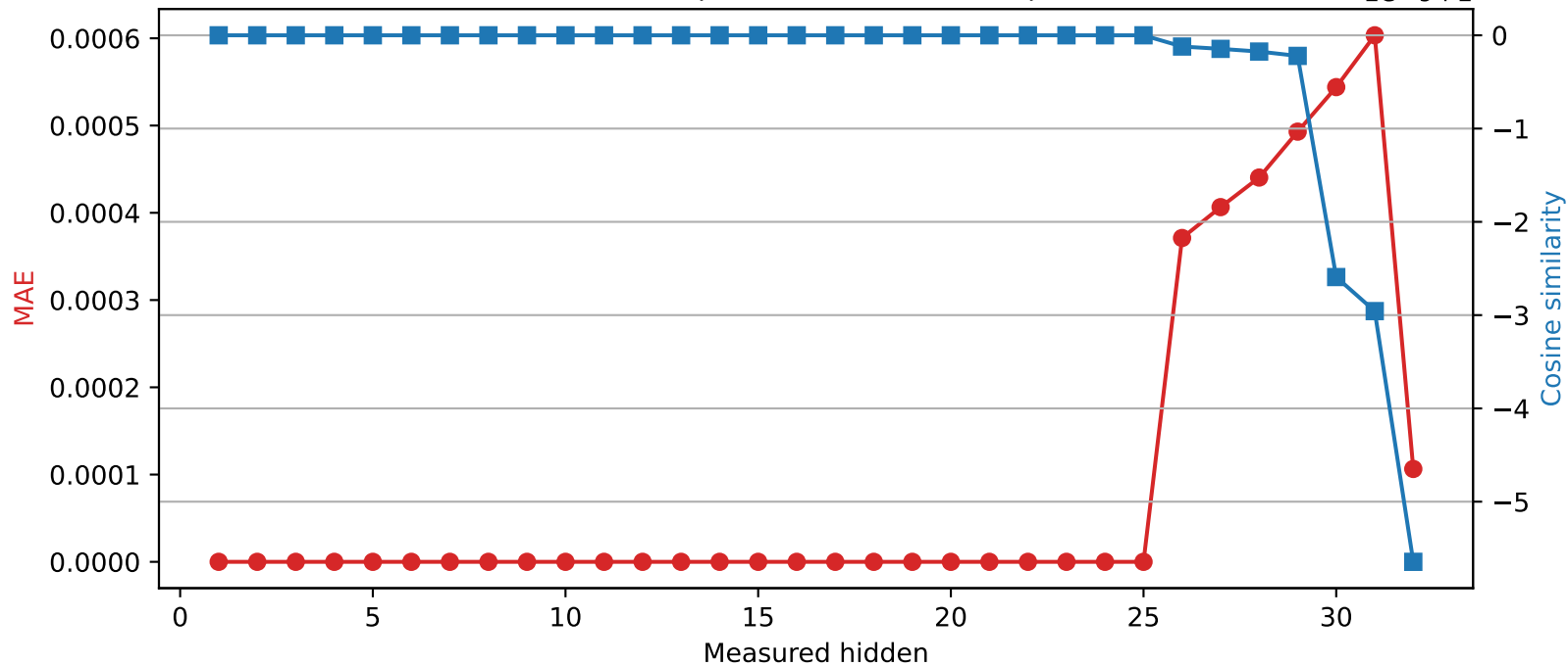
Phi-3-mini-4k-instruct | Quantized layer 25 | float32 \rightarrow int16
