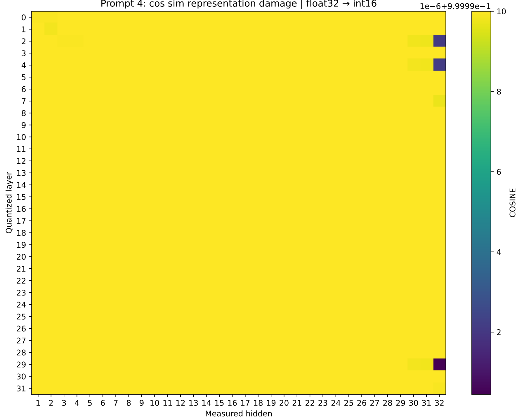
Phi-3-mini-4k-instruct Prompt 4: cos sim representation damage | float32 → int16
