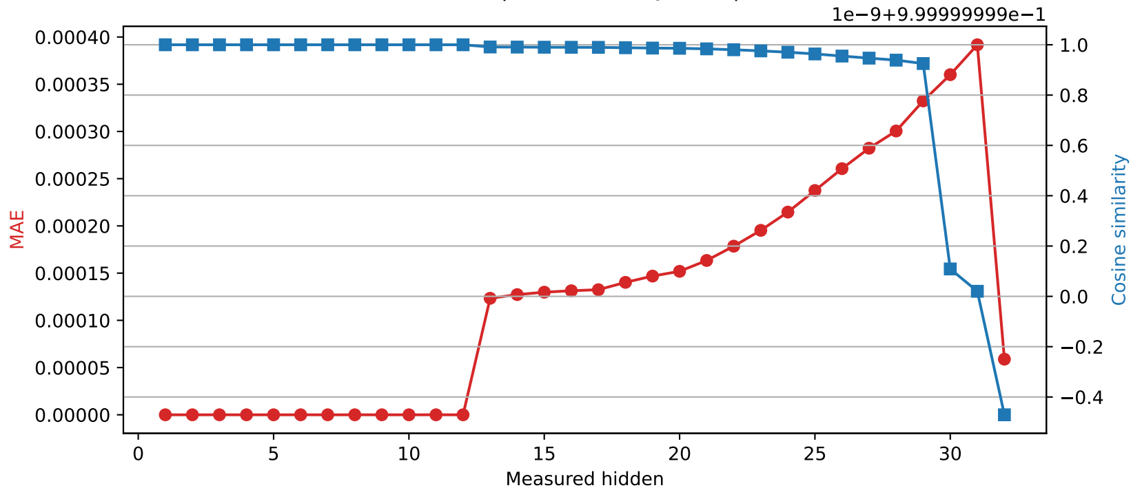
Phi-3-mini-4k-instruct | Quantized layer 12 | float32 → int16
