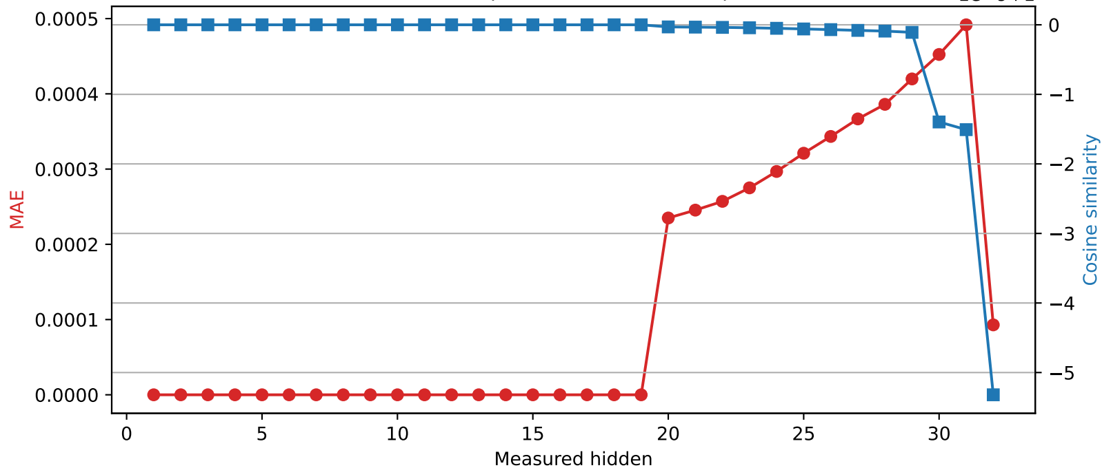
Phi-3-mini-4k-instruct | Quantized layer 19 | float32 \rightarrow int16
