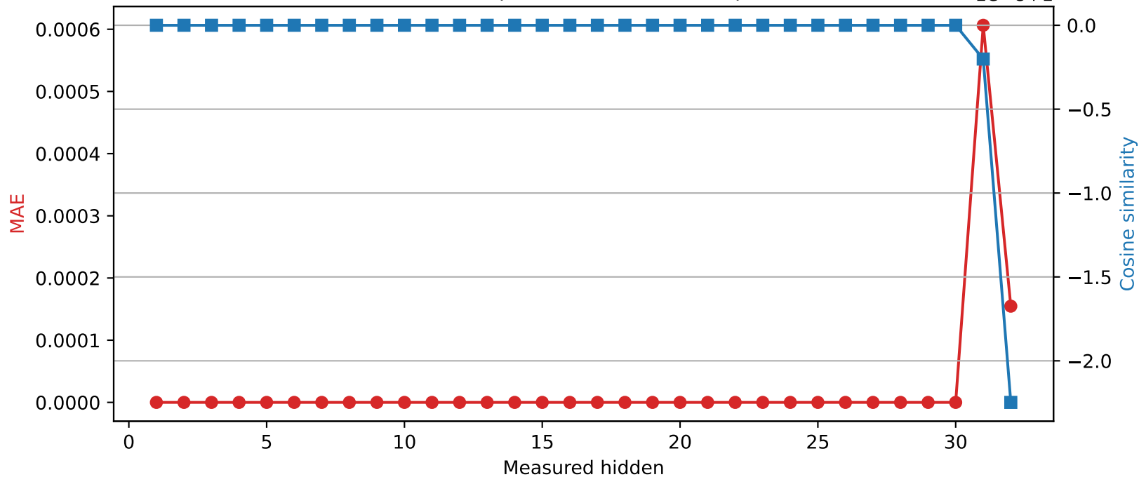
Phi-3-mini-4k-instruct | Quantized layer 30 | float32 \rightarrow int16
