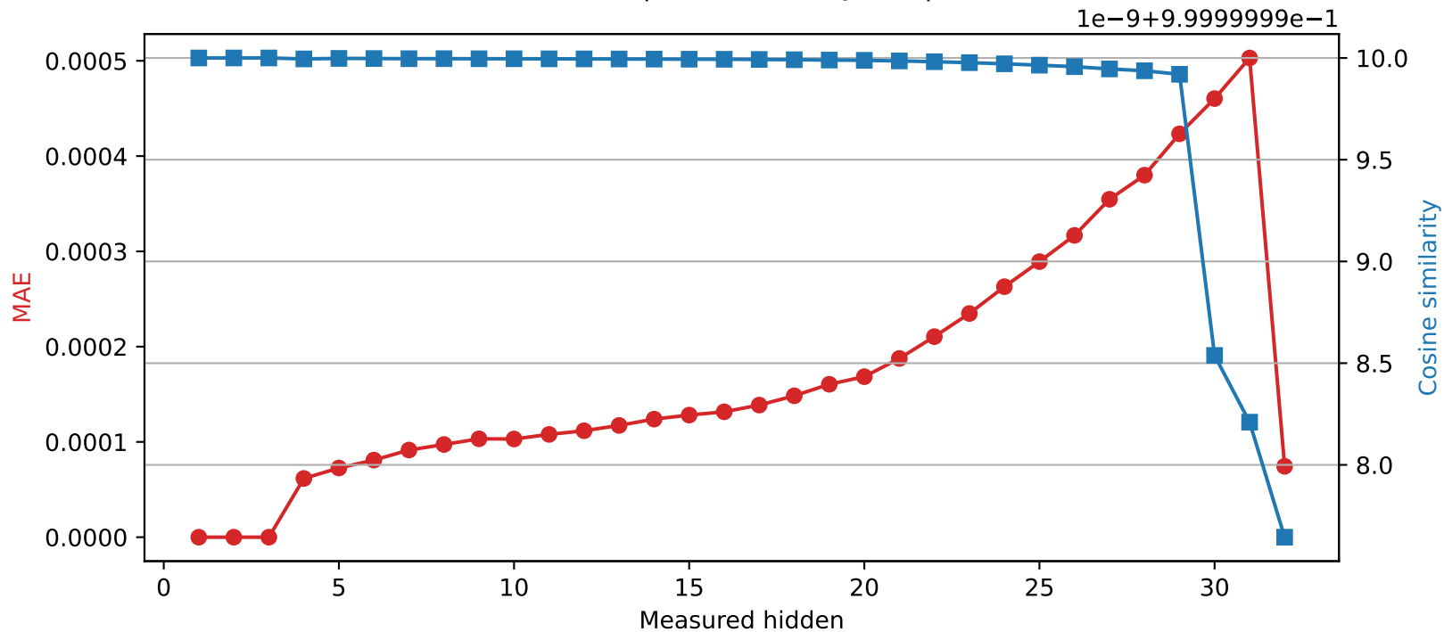
Phi-3-mini-4k-instruct | Quantized layer 3 | float64 → int16
