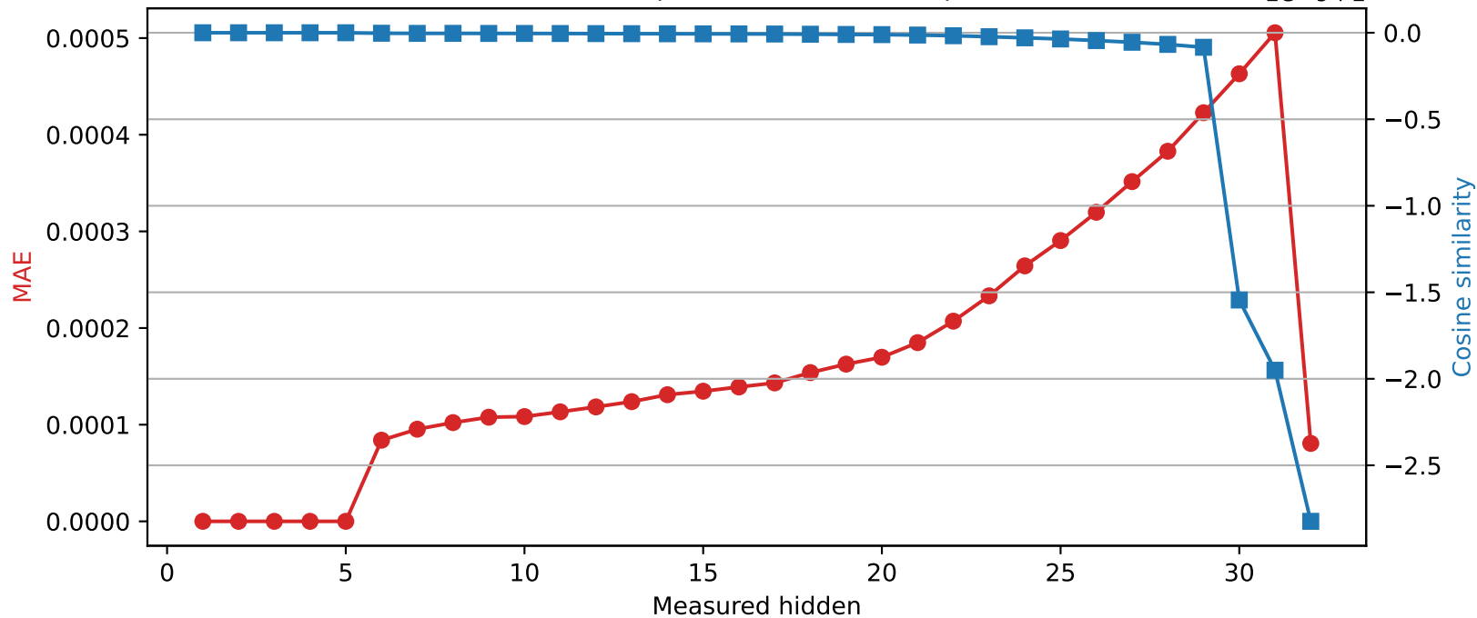
Phi-3-mini-4k-instruct | Quantized layer 5 | float64 → int16
