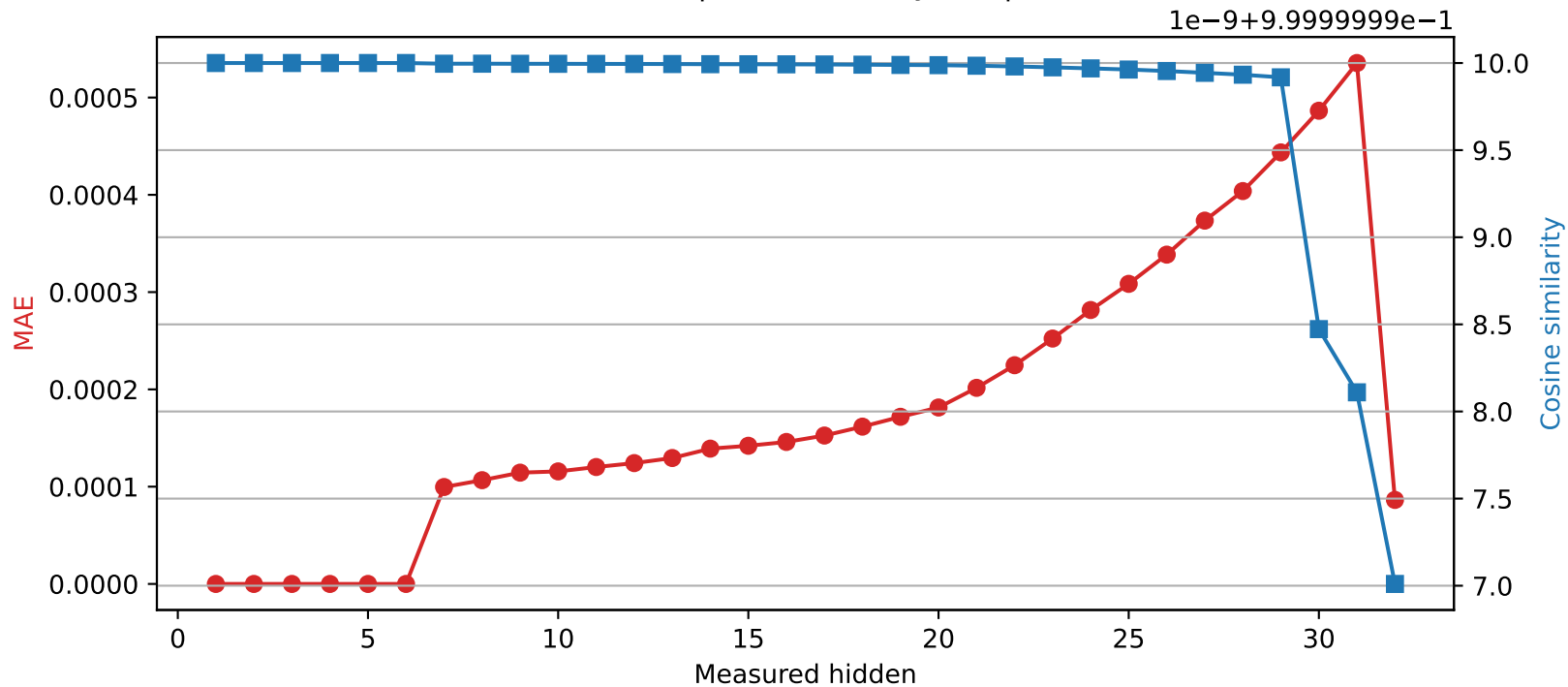
Phi-3-mini-4k-instruct | Quantized layer 6 | float64 → int16
