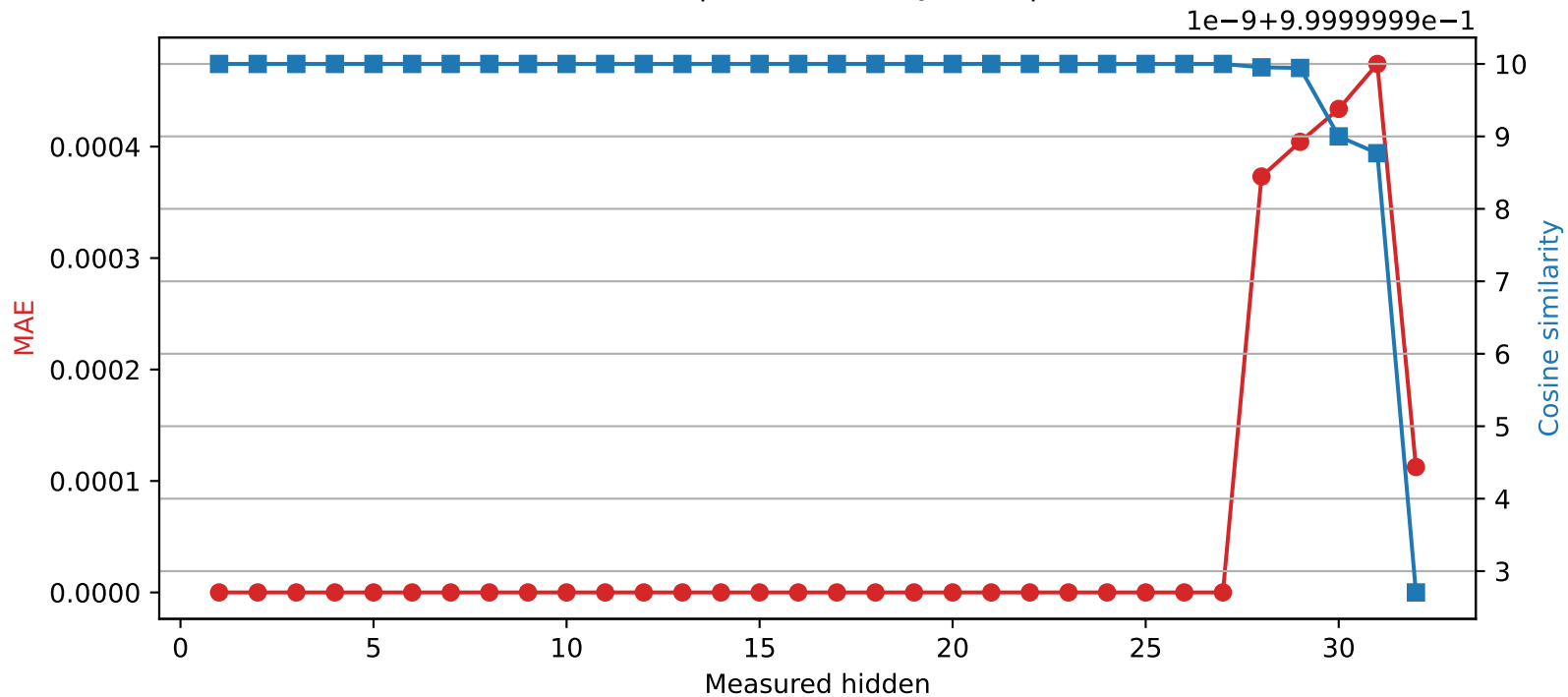
Phi-3-mini-4k-instruct | Quantized layer 27 | float64 → int16
