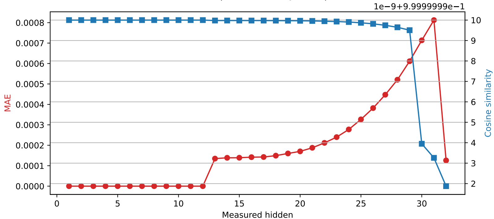
Phi-3-mini-4k-instruct | Quantized layer 12 | float64 → int16
