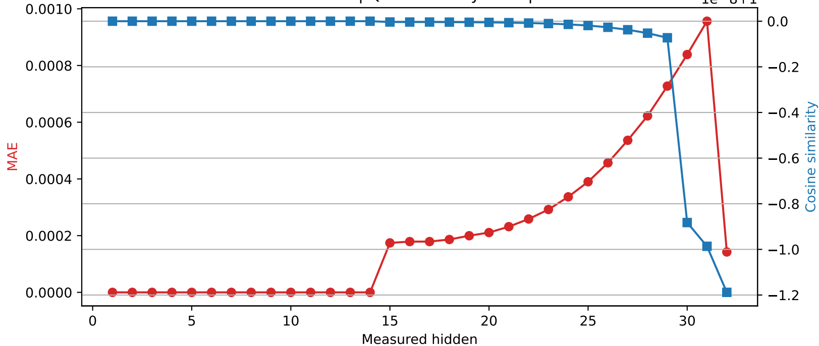
Phi-3-mini-4k-instruct | Quantized layer 14 | float64 → int16
