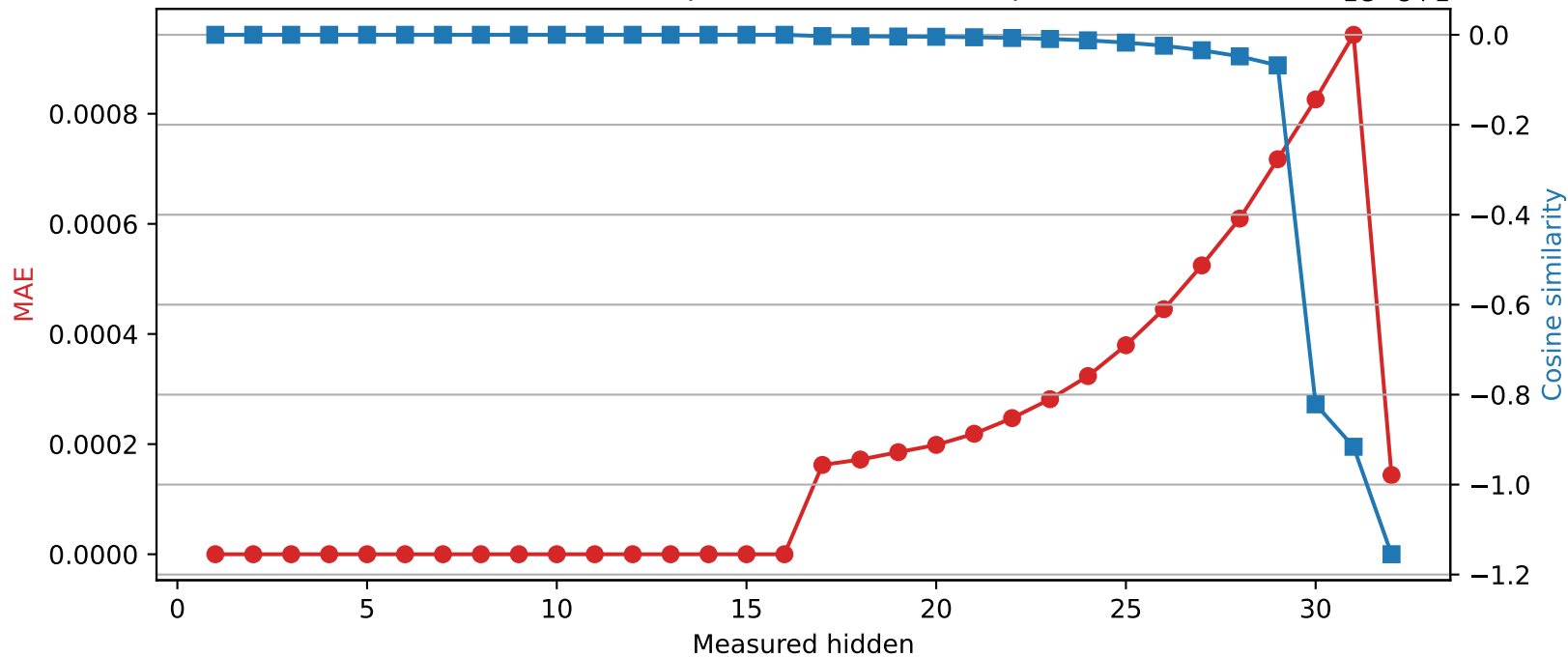
Phi-3-mini-4k-instruct | Quantized layer 16 | float64 → int16
