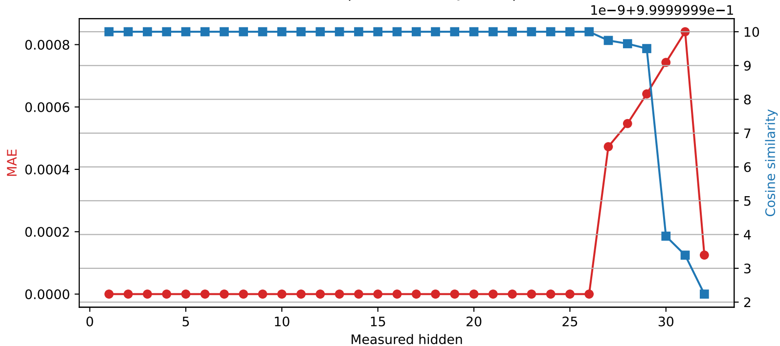
Phi-3-mini-4k-instruct | Quantized layer 26 | float64 → int16
