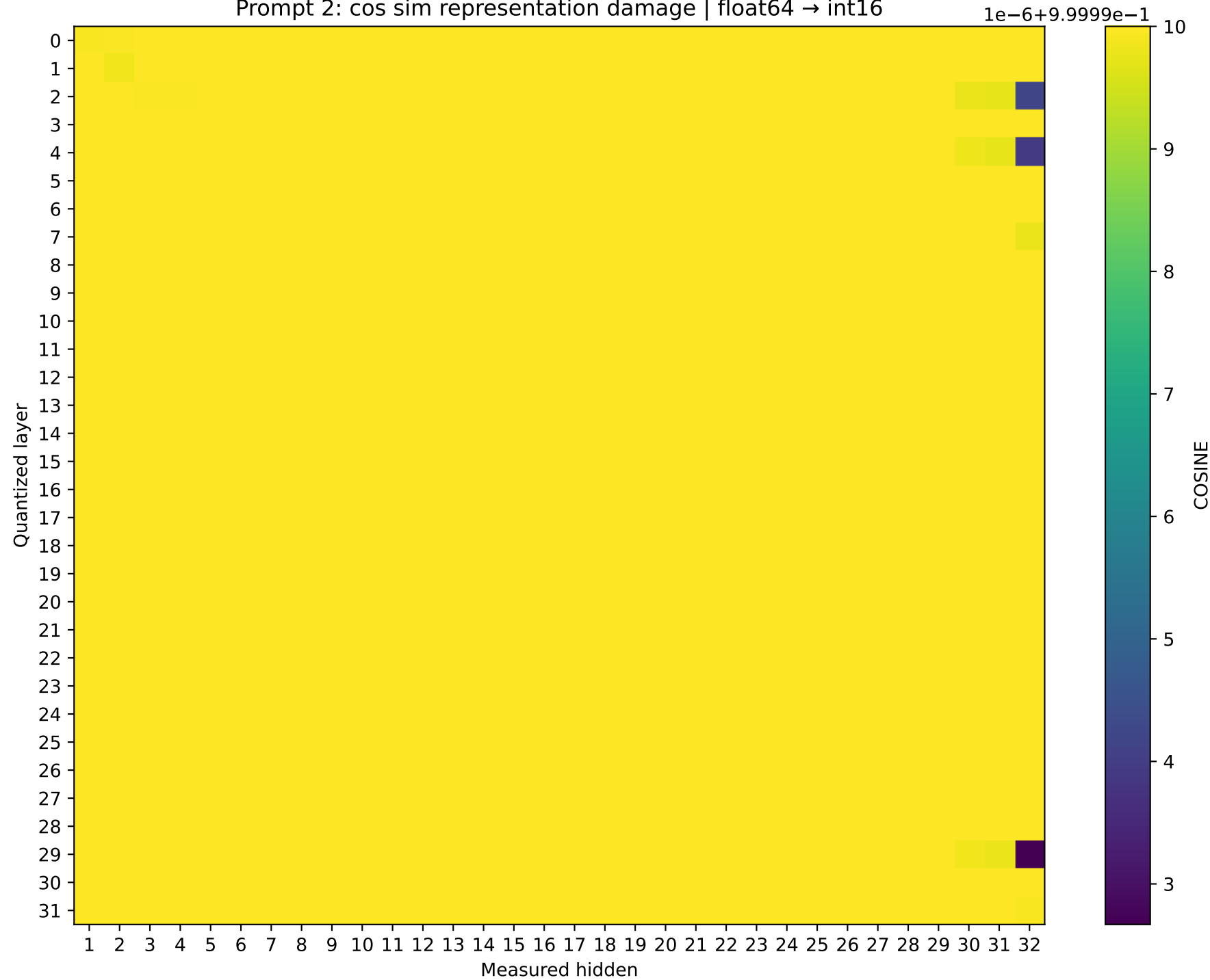
Phi-3-mini-4k-instruct Prompt 2: cos sim representation damage | float64 → int16
