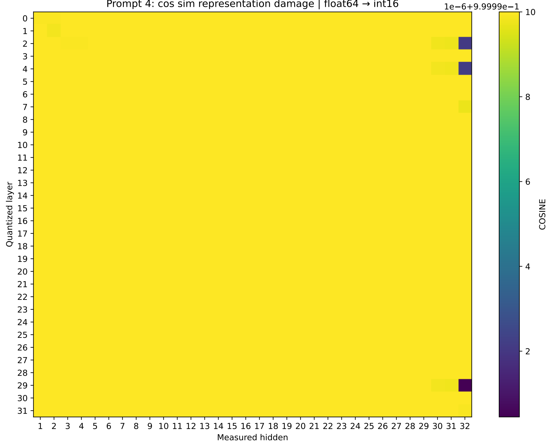
Phi-3-mini-4k-instruct Prompt 4: cos sim representation damage | float64 → int16
