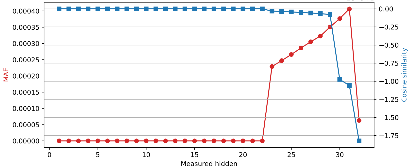
Phi-3-mini-4k-instruct | Quantized layer 22 | float64 → int16
