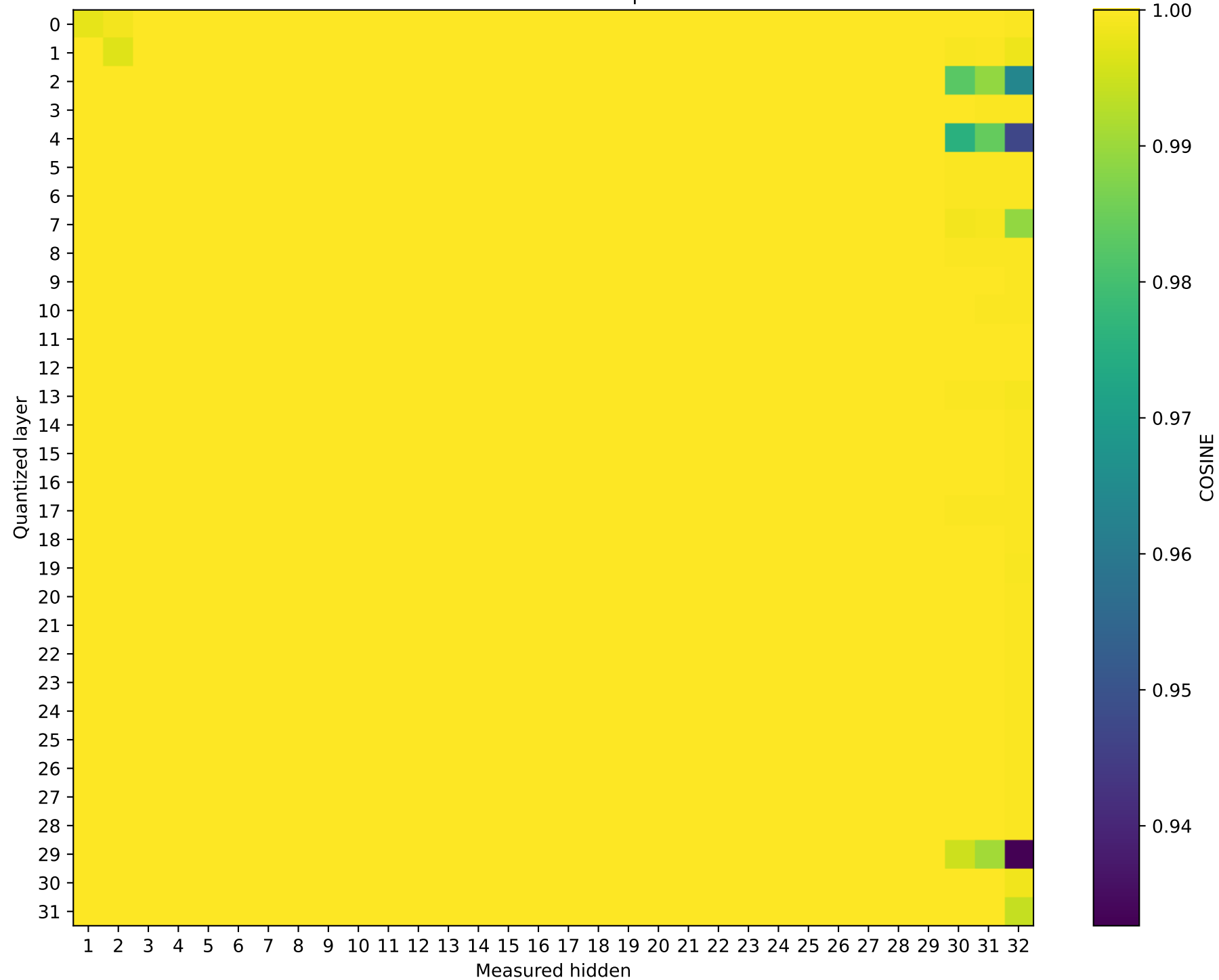
Model: Phi-3-mini-4k-instruct | float16 → int8
