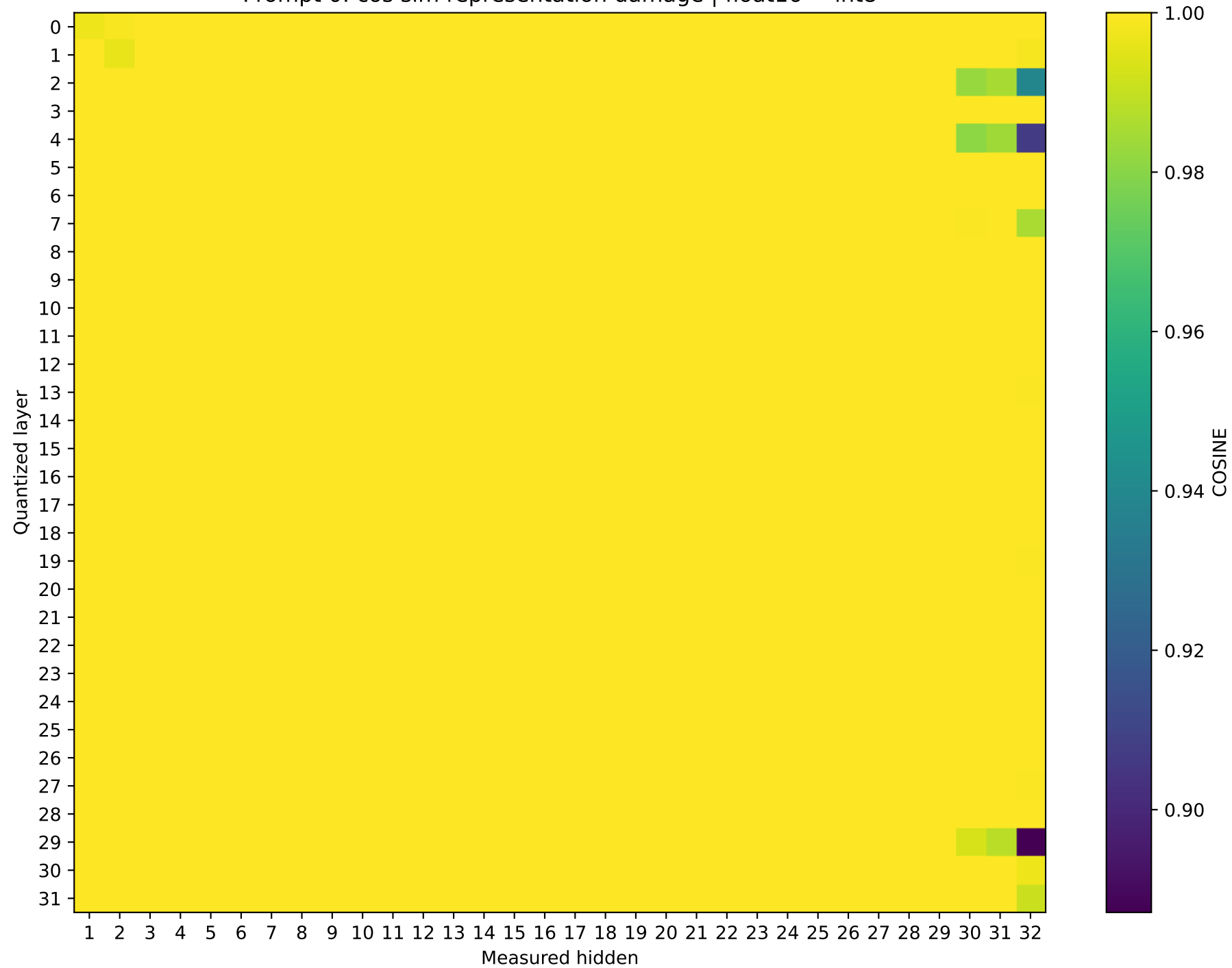
Phi-3-mini-4k-instruct Prompt 0: cos sim representation damage | float16 \rightarrow int8
