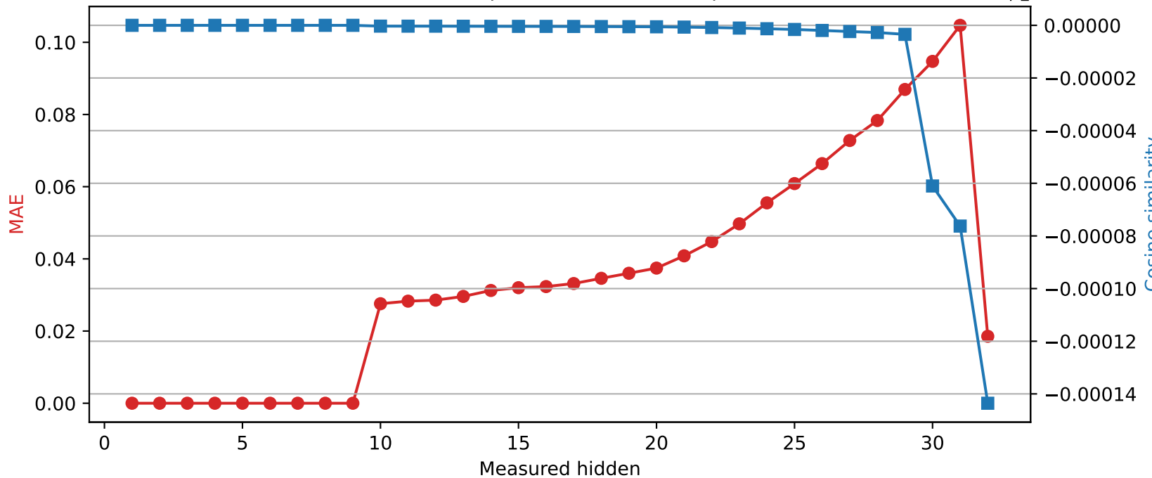
Phi-3-mini-4k-instruct | Quantized layer 9 | float16 \rightarrow int8
